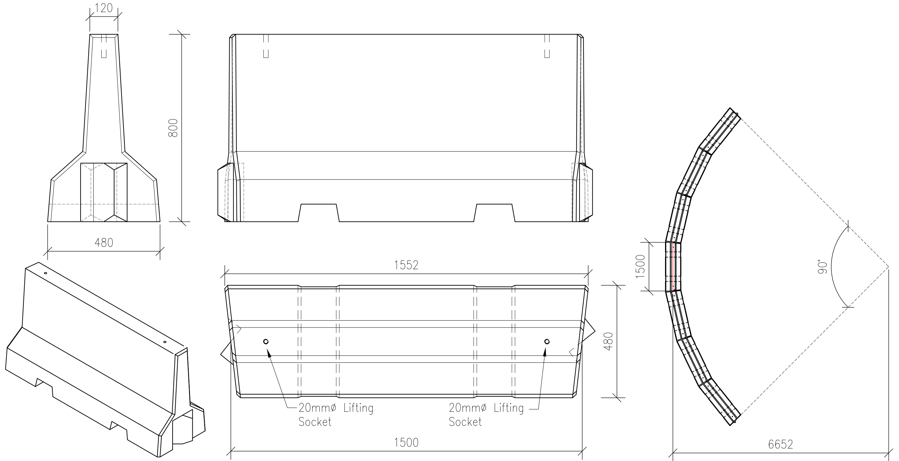
DOUBLE-SIDED CONCRETE CRASH BARRIER SECTIONS WITHOUT BACKING (FREE - STANDING)
